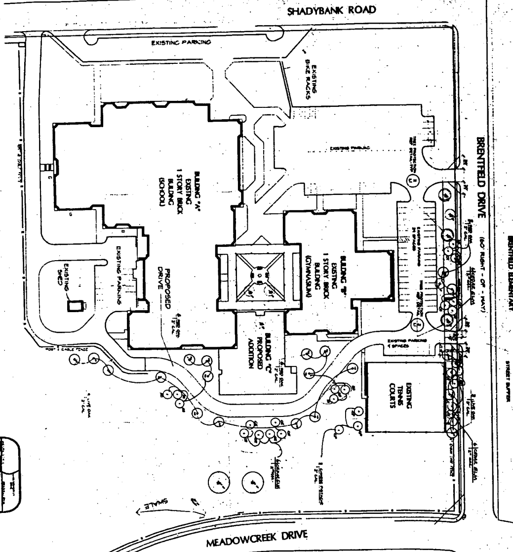
1 LANDSCAPE PLAN SCALE 1" = 40'-0"
